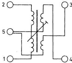
Fig. 3. Connection diagram
