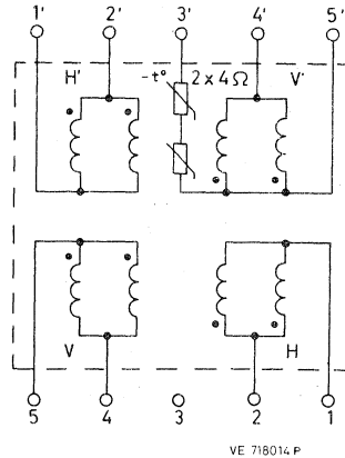
Fig. 3 Circuit diagram
