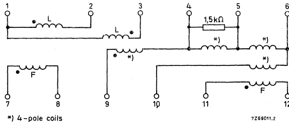
Fig. 2. Connection diagram.
