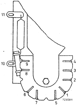
connecting pins
