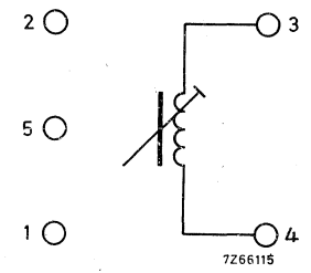
Fig.3 Connection diagram
