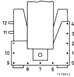
connecting pins
