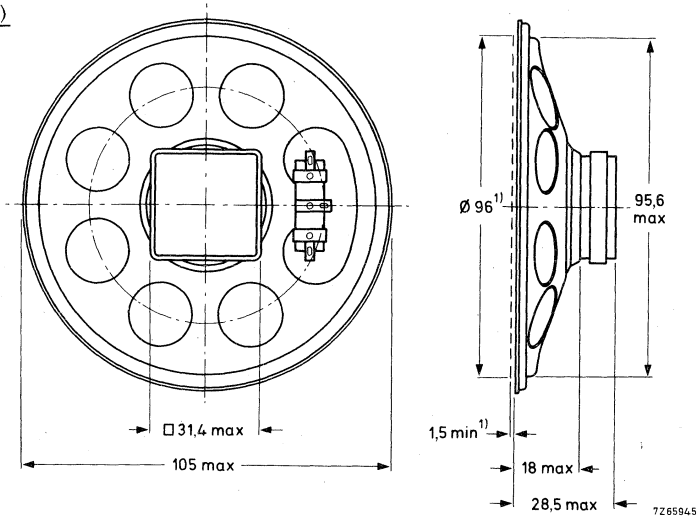
Fig. 1a Round flange version
