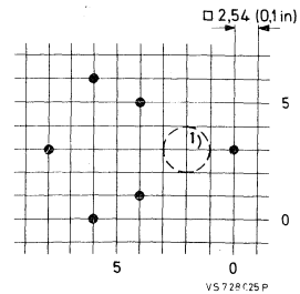
Fig. 2 Hole pattern for mounting on a printed-wiring board. Hole diameter 1, 3 + 0, 1
