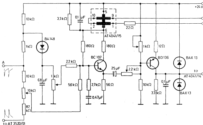
Circuit diagram for AT4041/15
