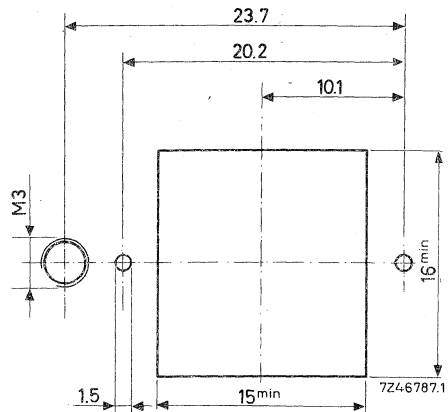
Fig. 4. Hole pattern for mounting on a chassis.
