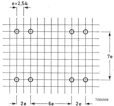
Fig. 3 Hole pattern for mounting on a printed-wiring board. Hole diameter 1.3 + 0,1 mm.
