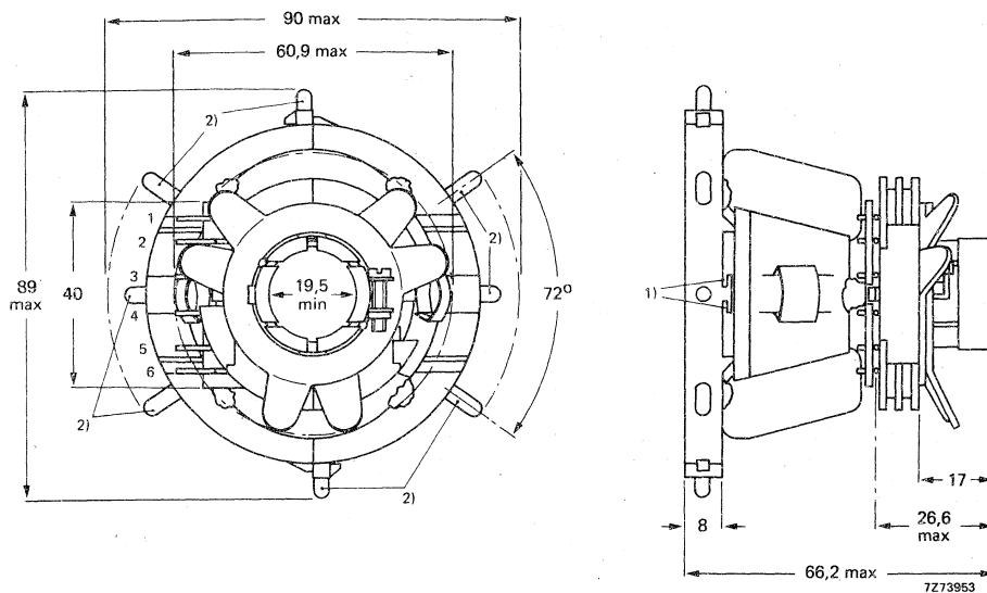
Fig. 1. 1) For fitting plastic-bonded FXD magnet strips, catalogue number 3122 137 10160. 2) For fitting plastic-bonded FXD magnets, catalogue number 3122 104 94120.
