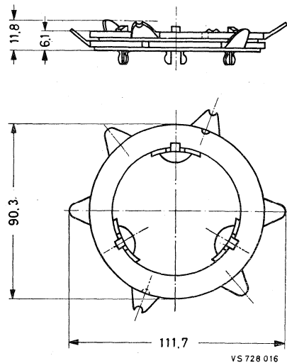
Fig. 5. Dimensions in mm of the purity ring AT1061
