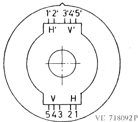
Fig. 2 Terminal location
