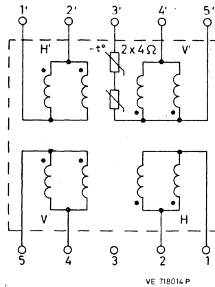
Fig. 3. Circuit diagram
