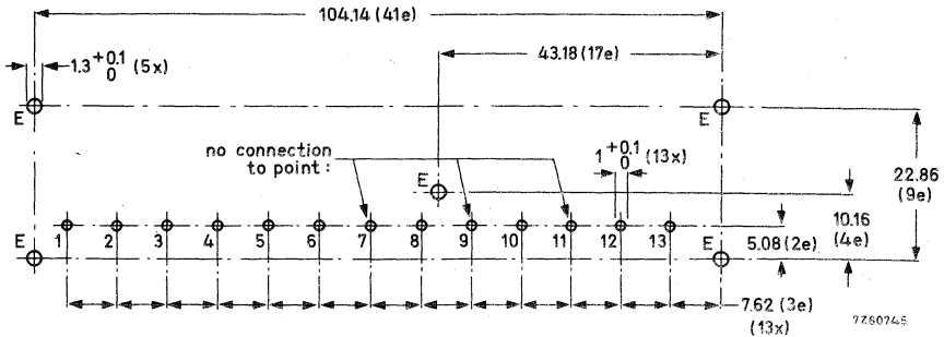
Fig. 3. Piercing diagram viewed from solder side of board; e = 2,54 \text{ mm} (0,1 \text{ in}) .
