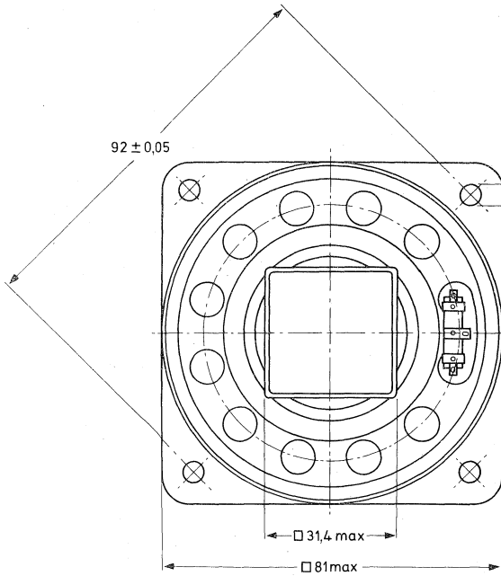
Fig. 1b Square flange version
