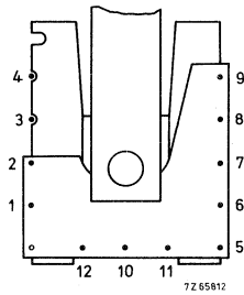
connecting pins
