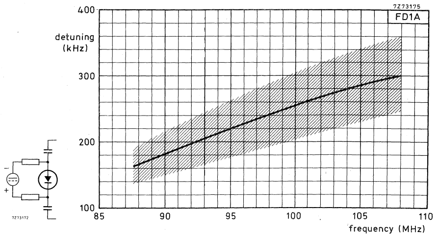
Fig. 6. Detuning as a function of signal frequency at a control voltage change from 0 to +400 mV.
