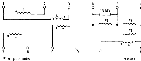
Fig. 2. Connection diagram.
