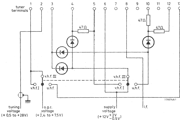
Fig. 15. Connection diagram with two switches. All diodes: BAX13, BA217 or comparable silicon diodes.
