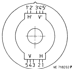
Fig. 2. Terminal location
