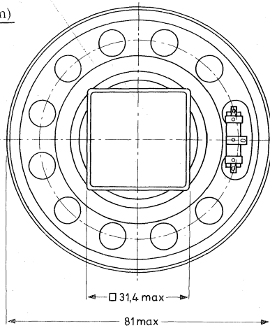
Fig. 1a Round flange version
