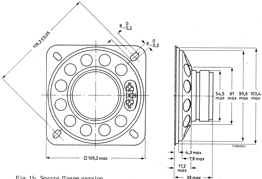
Fig. 1b Square flange version
