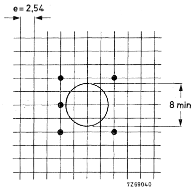
Fig. 2 Hole pattern for mounting on a printed-wiring board, hole dia 1,3 + 0,1 mm
